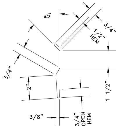
RAKE CLOSURE
