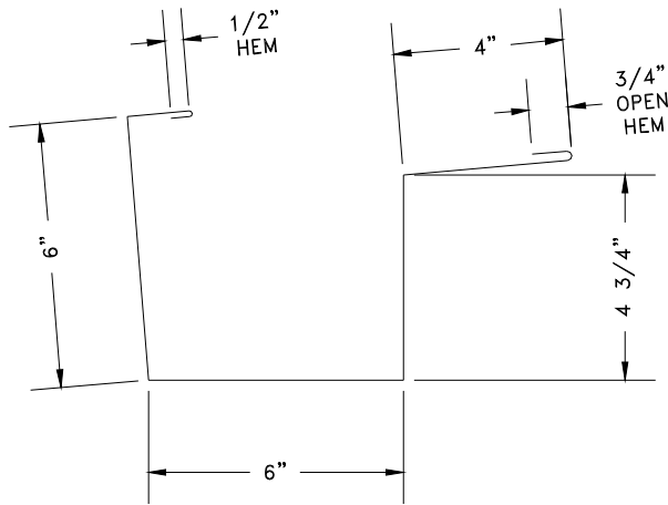
GUTTER
