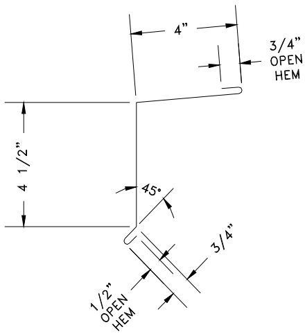
EAVE
