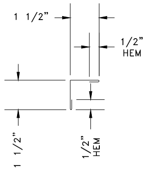
HIGH EAVE
