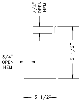
RAKE TRANSITION
